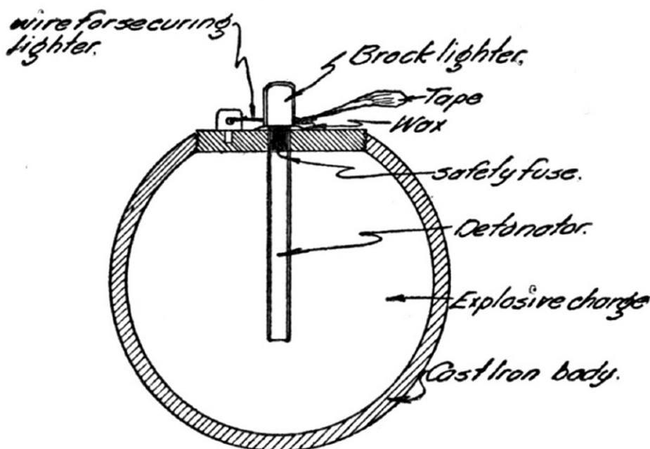
SECTION. Diameter of Grenade 3"
